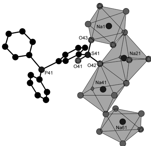
Figure 3. Diagram of one of the four TPPMS Na molecules and the four crystallographically independent oxygen coordinated sodium atoms. The hydrogen atoms and the minor components of the disordered water molecules are omitted for clarity. The NaO 6 octahedra are connected through shared vertices and edges. Oxygen atoms that belong to sulfonate groups of TPPMS are marked with front ellipses.
