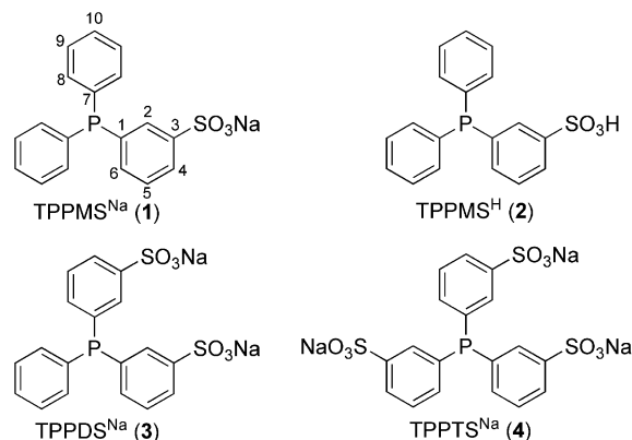
Scheme 1. Sulfonated triphenylphosphanes.
