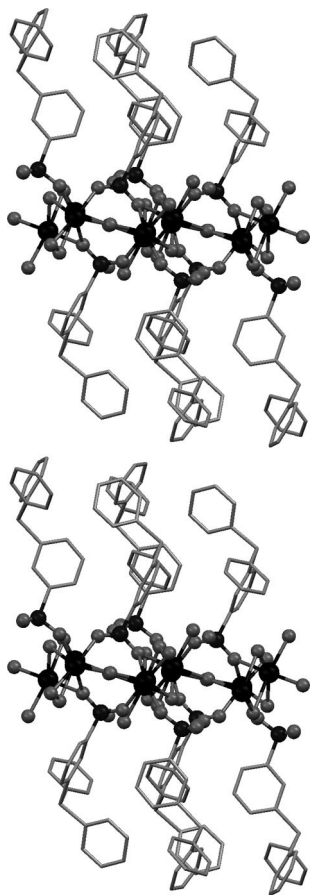
Figure 2. Packing diagram of sodium triphenylphosphane monosulfonate. Only the major components of the disordered water molecules are shown.
