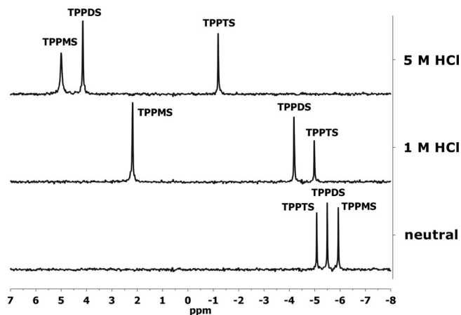
Figure 4. Downfield shift and peak intensities of sulfonated phosphanes in the ^{31}\text{P}\{^1\text{H}\} NMR spectra at different pH values.
