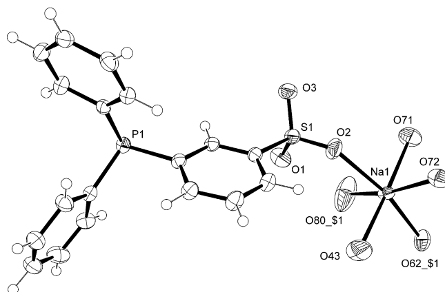
Figure 1. ORTEP presentation of one out of four crystallographic independent TPPMS Na molecules including all five other oxygen atoms that are coordinated to Na1. Ellipsoids are drawn at 50% probability level. Used symmetry operator: $1: -x - 1, -y - 2, -z + 1 . O43 and O62_$1 are oxygen atoms of other sulfonate groups whereas O71, O72 and O80_$1 are oxygen atoms of water molecules. Hydrogen atoms of water molecules and one disordered water molecule were omitted for clarity.
